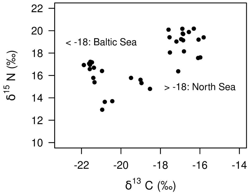
Fig. 3. Stable isotope values of 33 red-throated diver feather samples assigned to the region where they were moulted. Data points show feathers of 16 individuals moulted in the Baltic Sea and 17 individuals that moulted in the North Sea.
